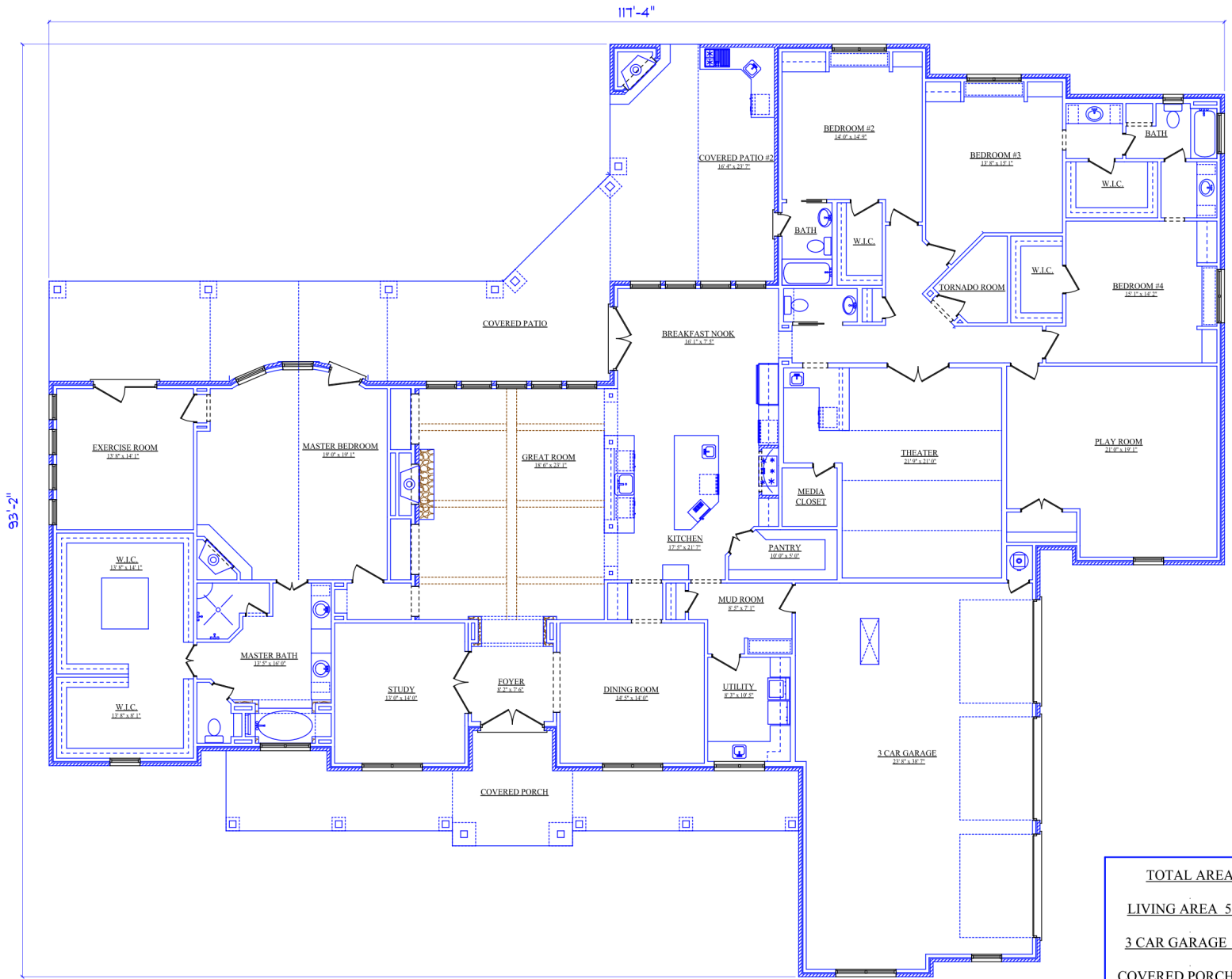
FLOOR PLAN
