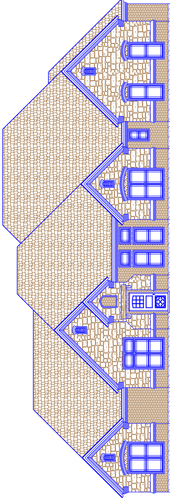
○ FRONT ELEVATION
