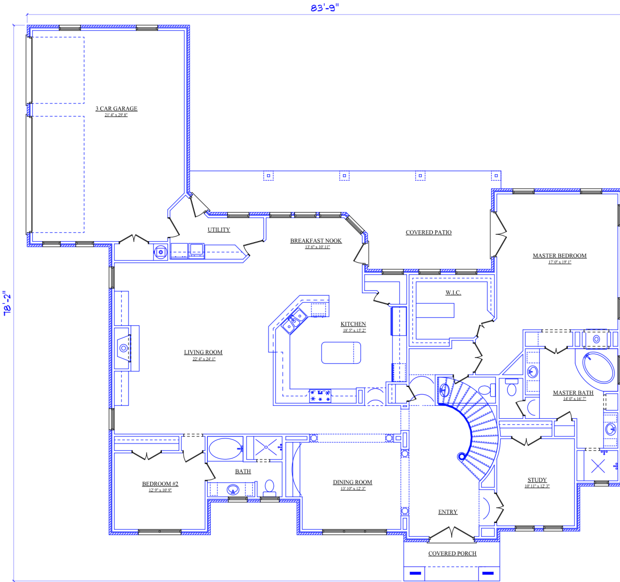
FLOOR PLAN
