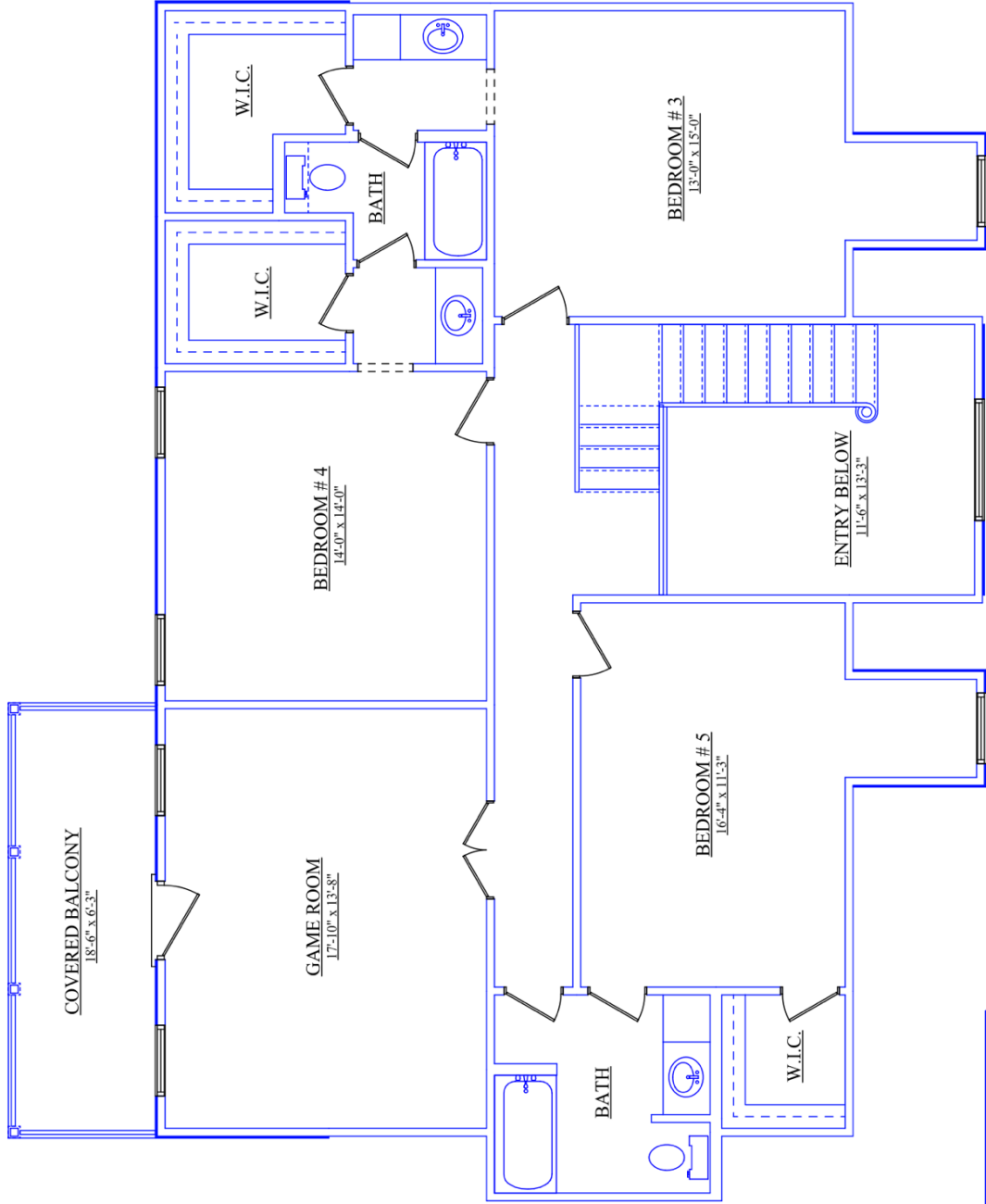
UPPER FLOOR PLAN
