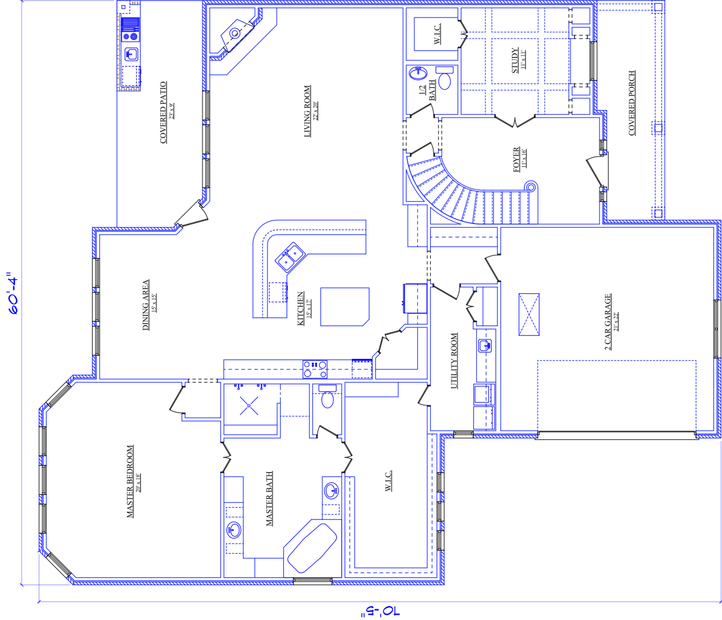
FLOOR PLAN
