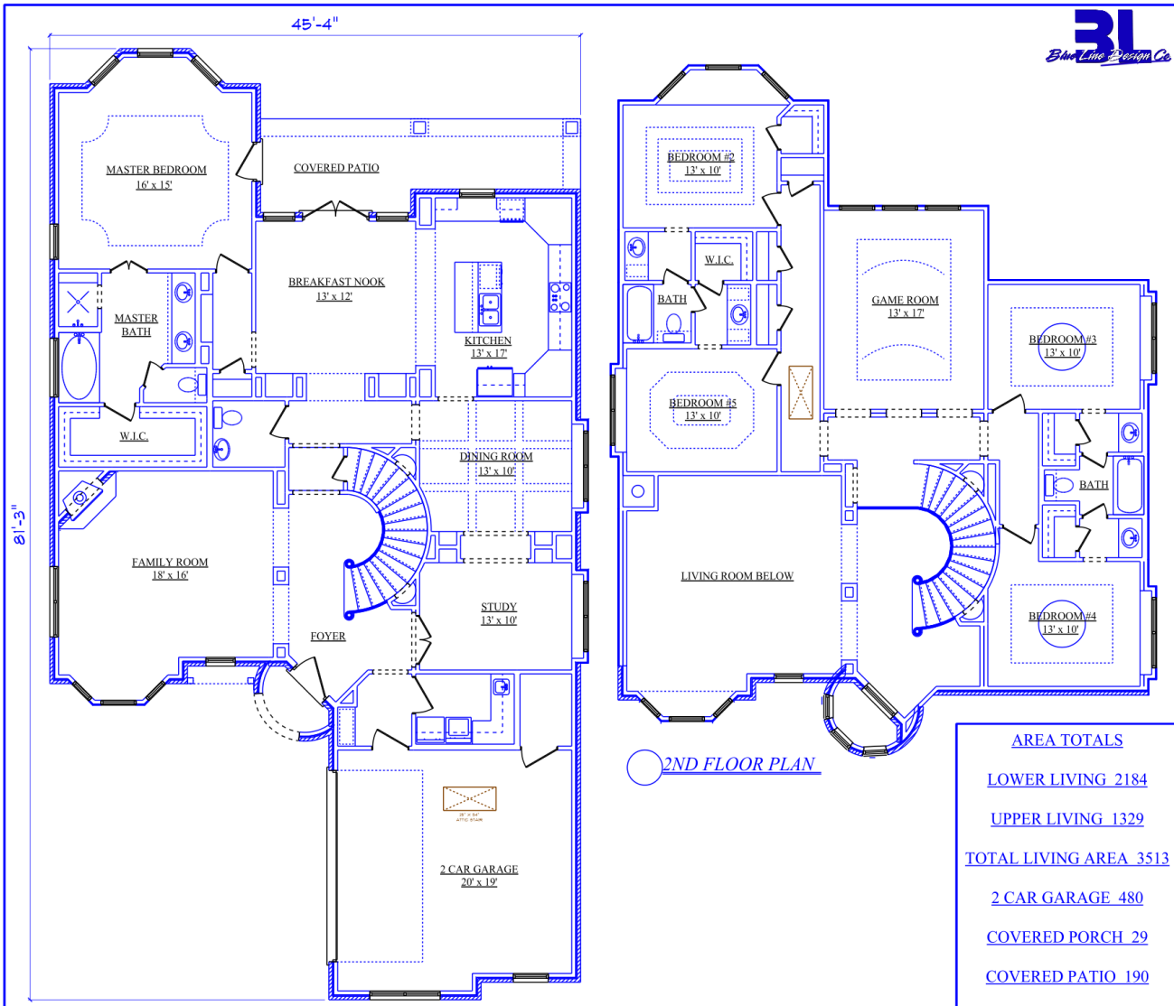
FLOOR PLAN
