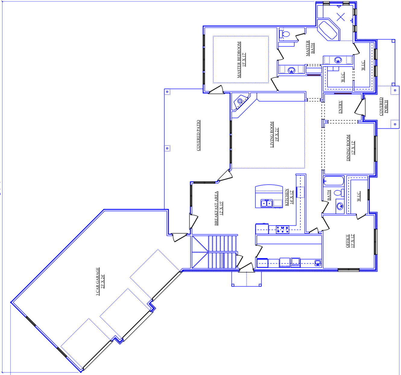
FLOOR PLAN
