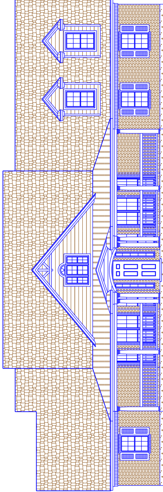
FRONT ELEVATION
