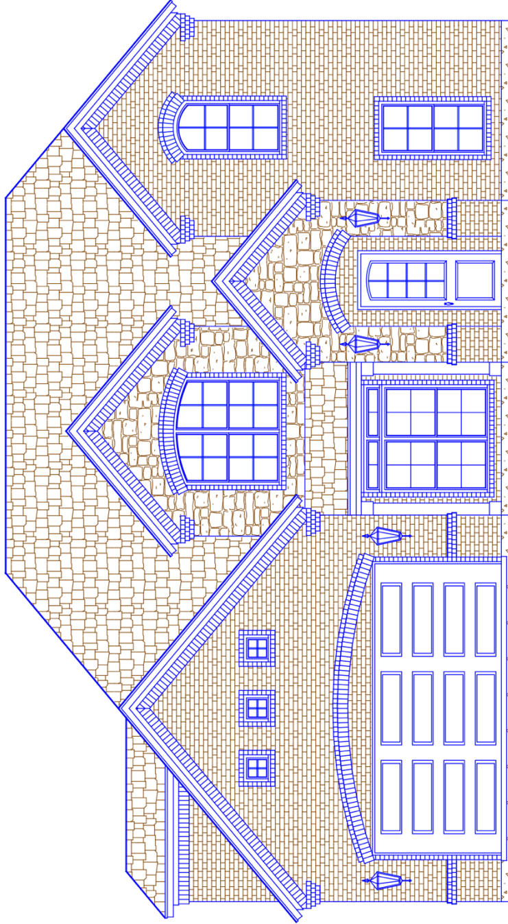
FRONT ELEVATION
