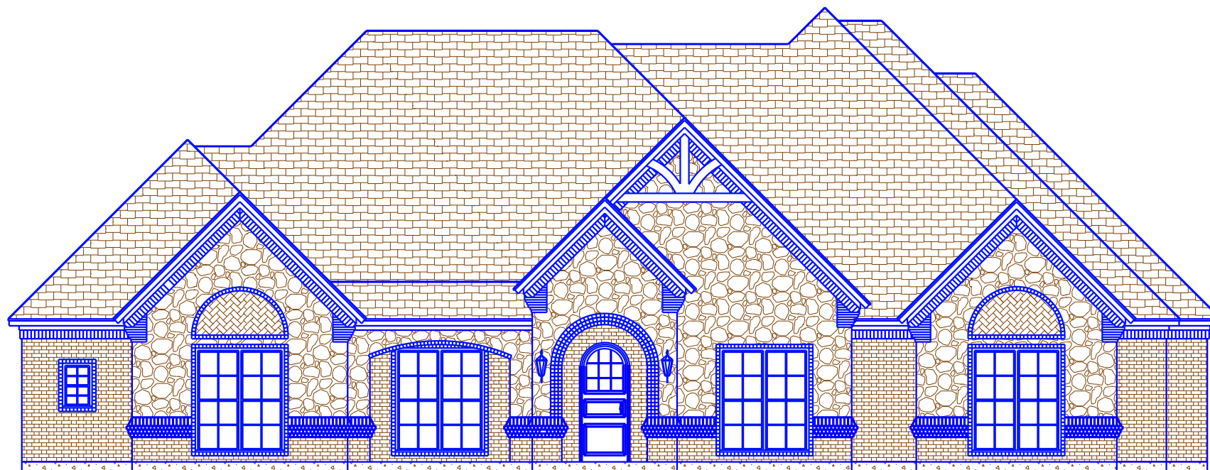
○ FRONT ELEVATION
