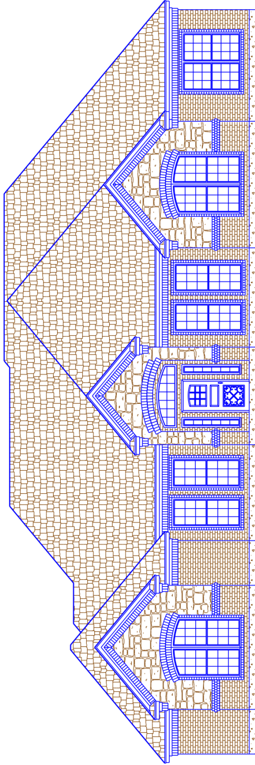
○ FRONT ELEVATION
