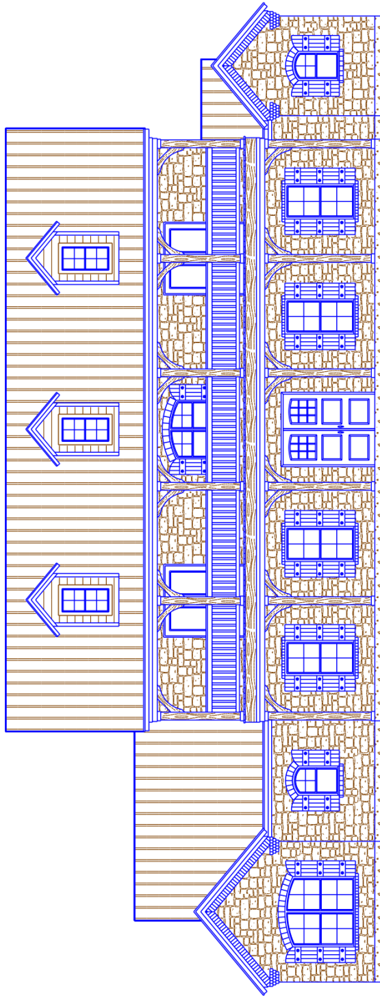
FRONT ELEVATION
