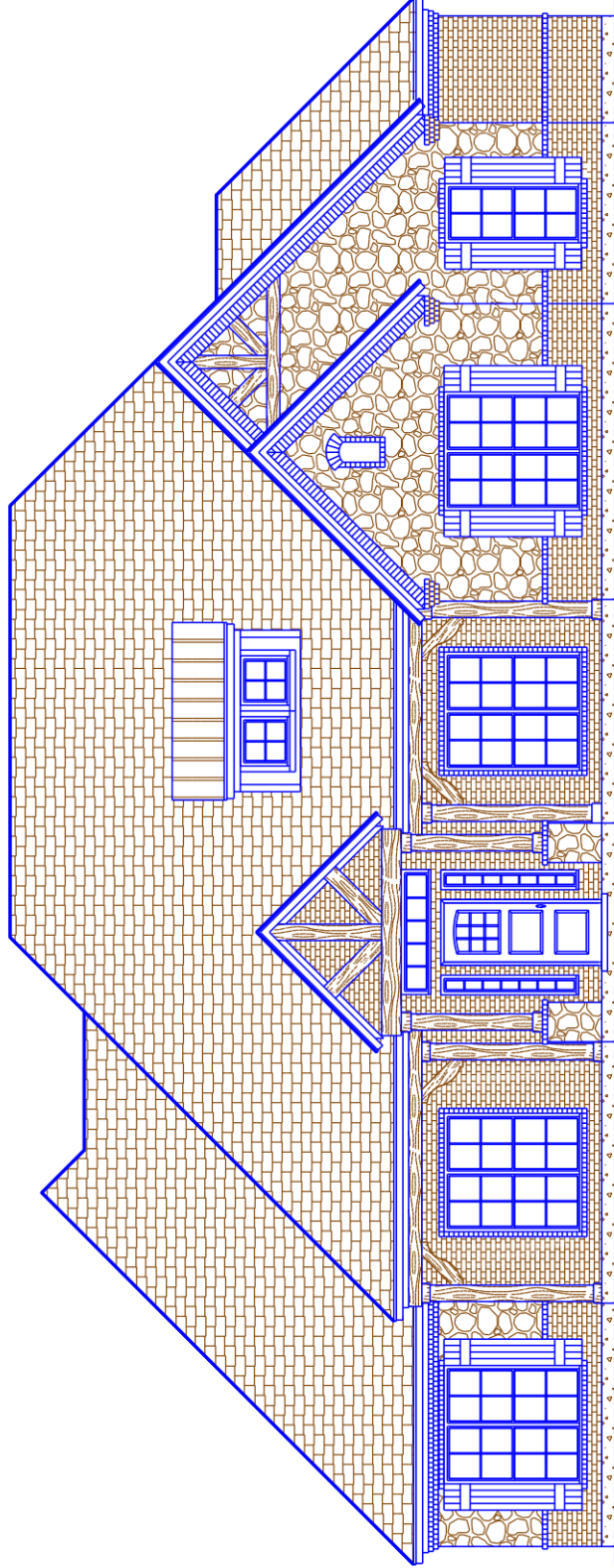
FRONT ELEVATION
