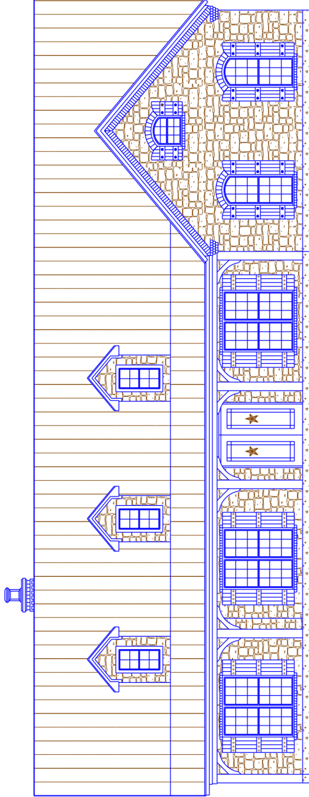
FRONT ELEVATION
