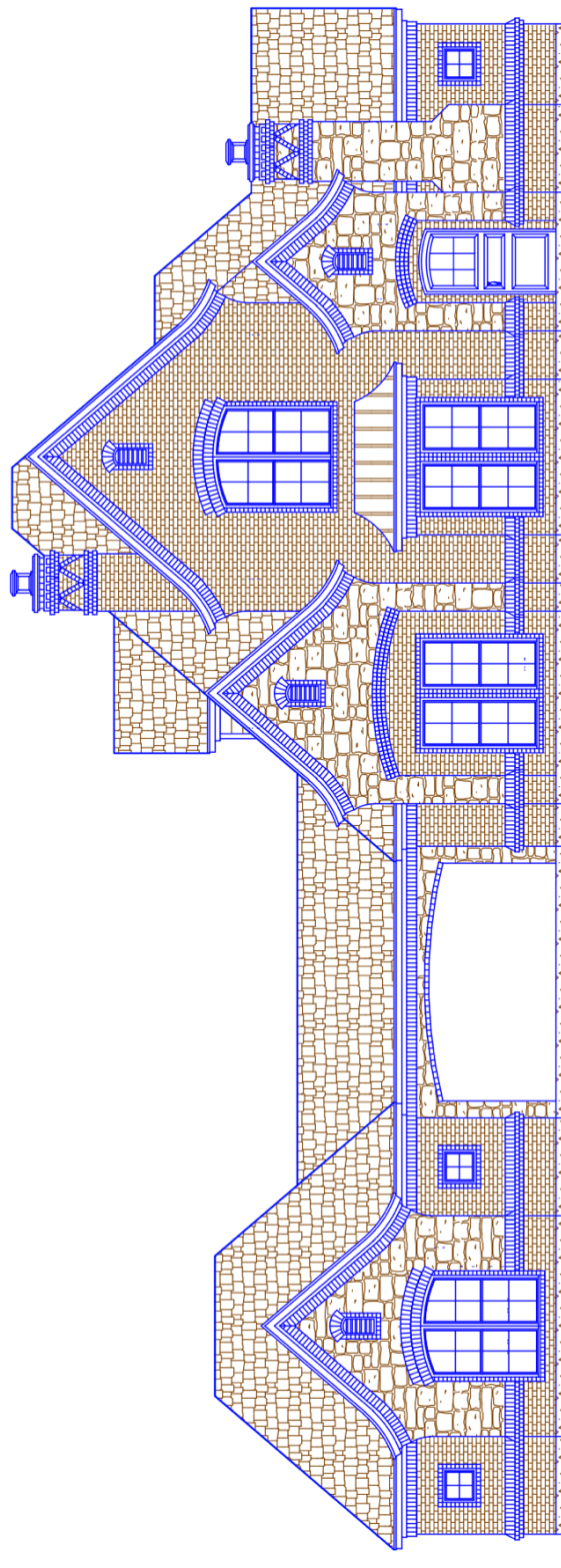
FRONT ELEVATION
