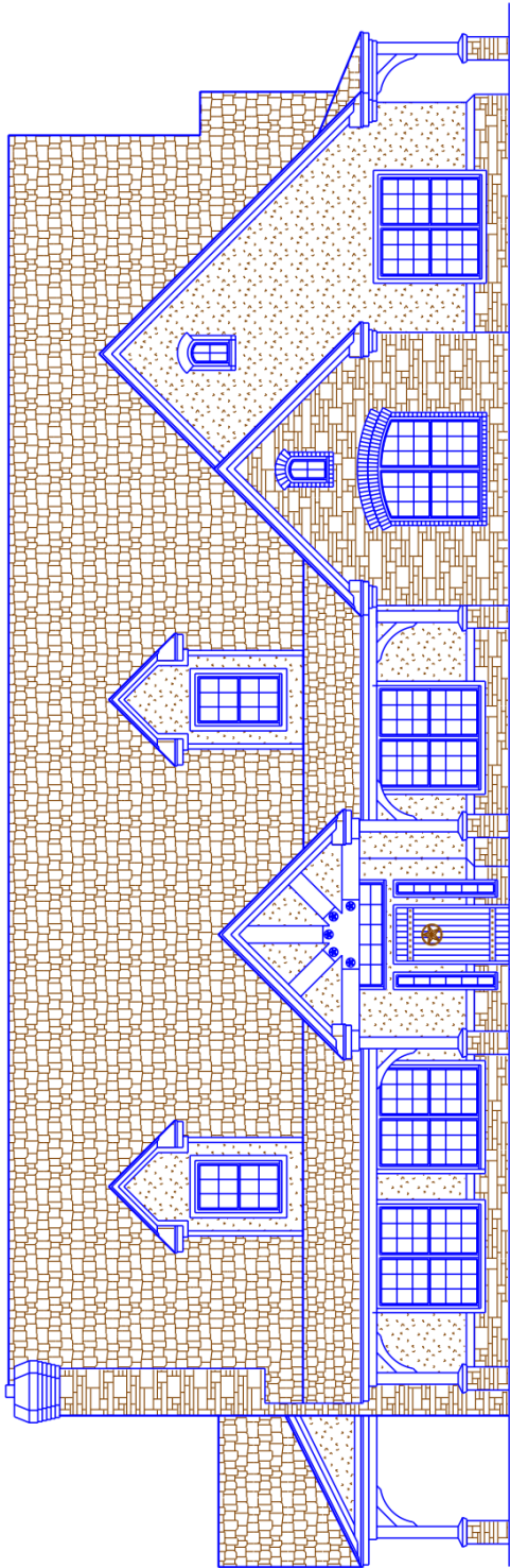
FRONT ELEVATION
