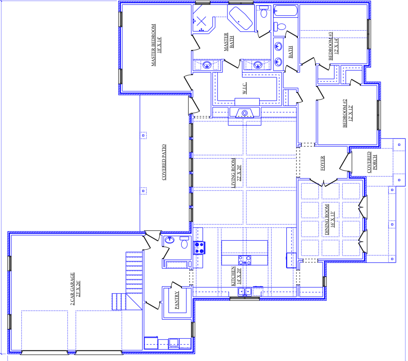
FLOOR PLAN
