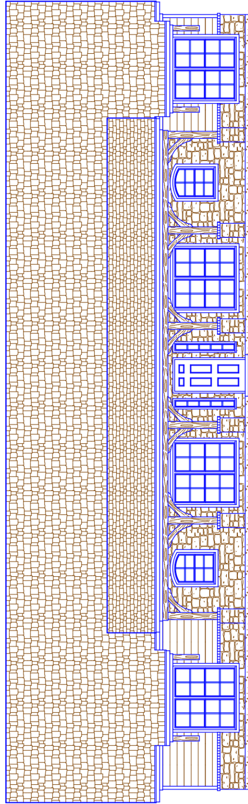
FRONT ELEVATION
