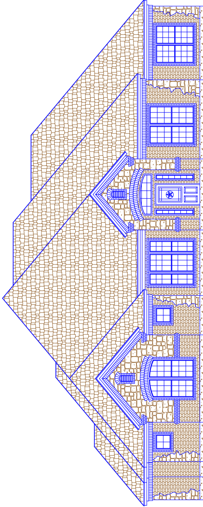
FRONT ELEVATION
