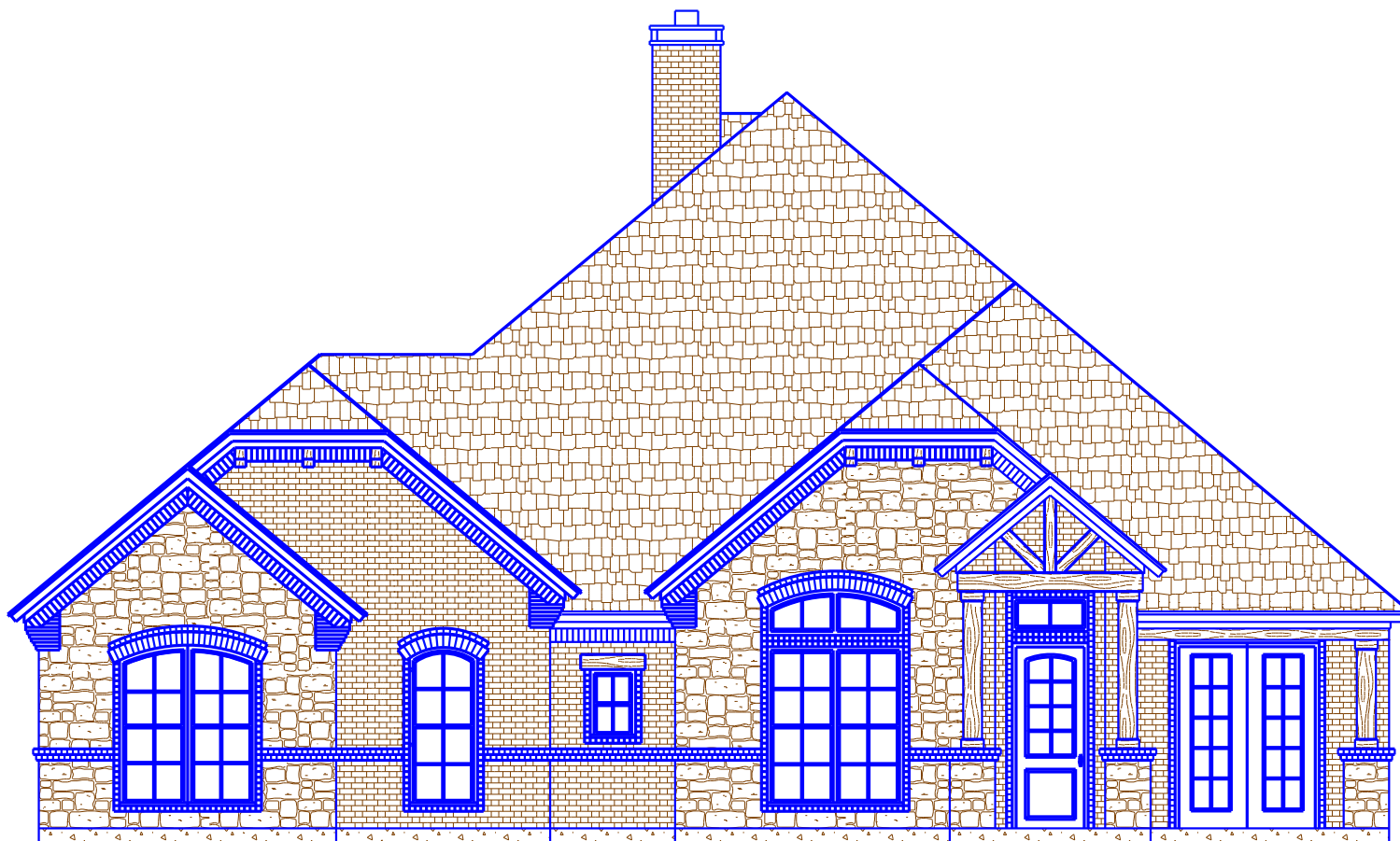
○ FRONT ELEVATION
