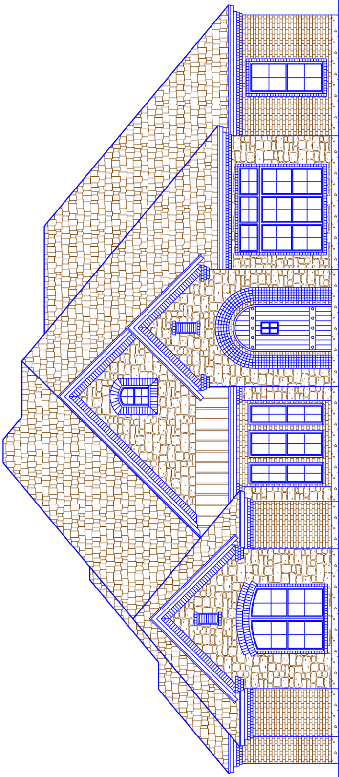
FRONT ELEVATION
