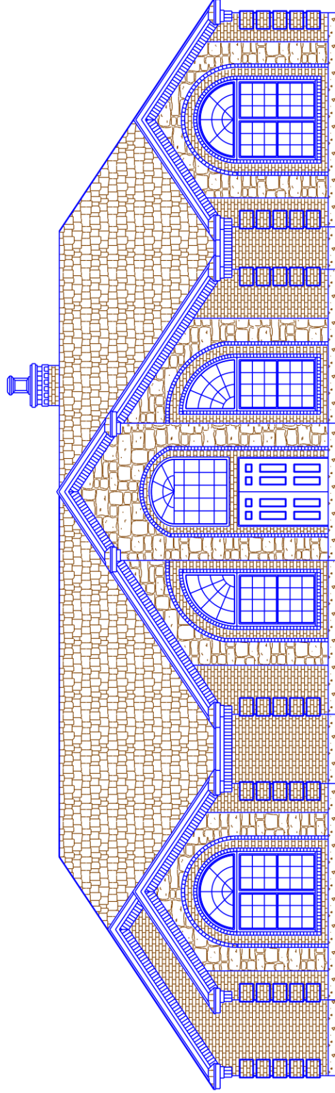
○ FRONT ELEVATION
