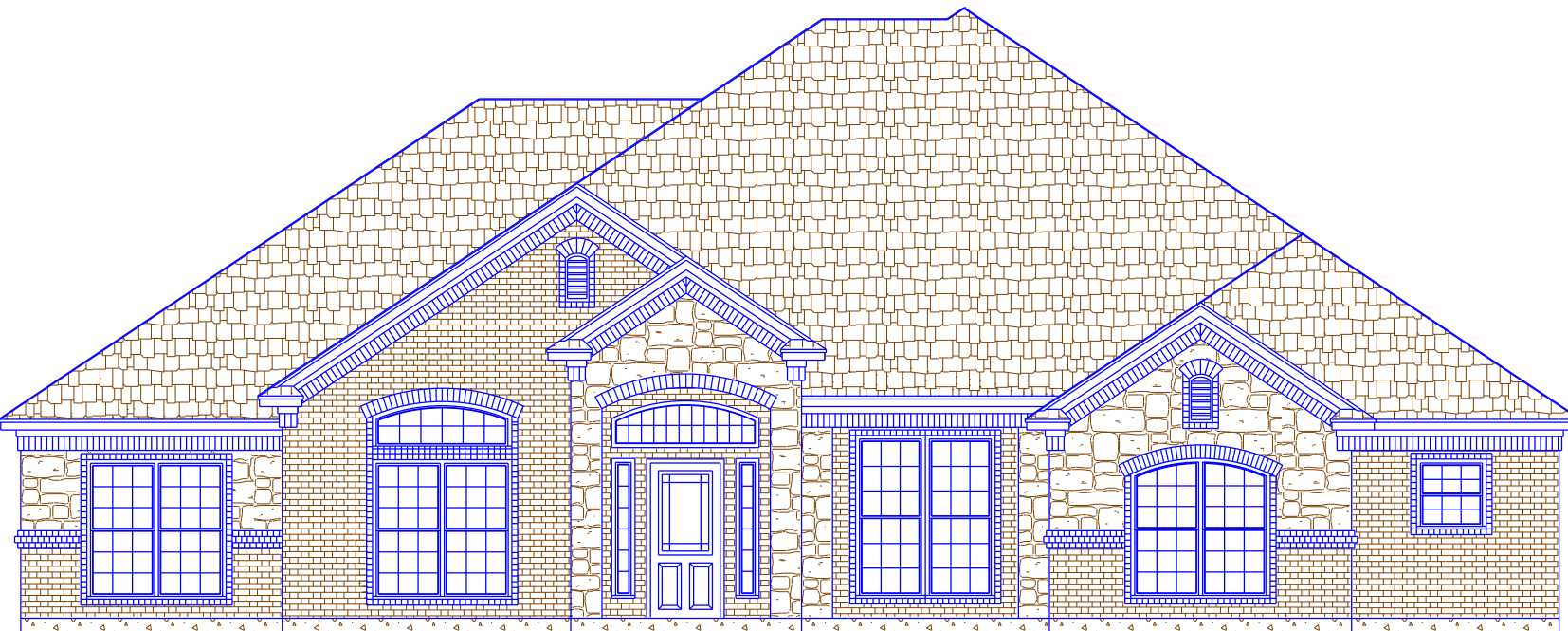
○ FRONT ELEVATION
