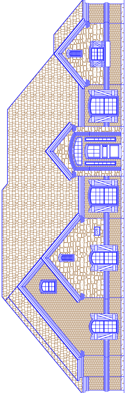
FRONT ELEVATION
