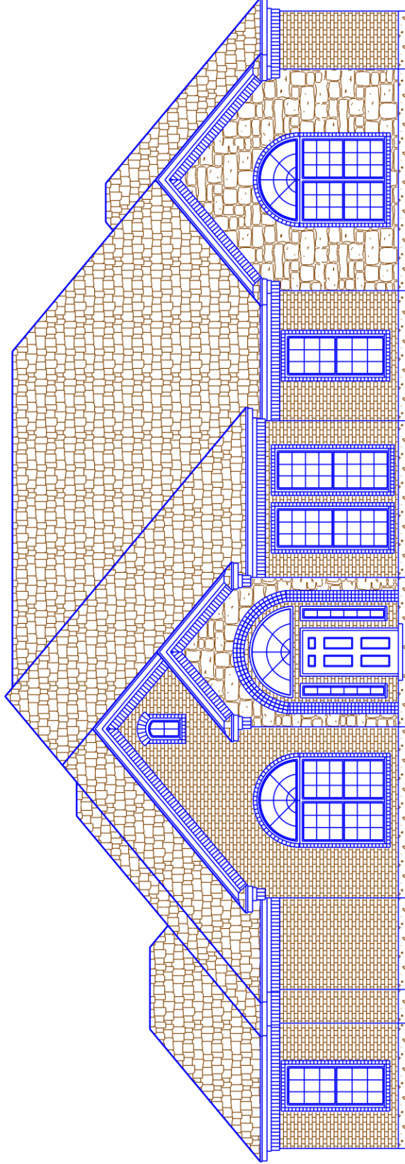
FRONT ELEVATION
