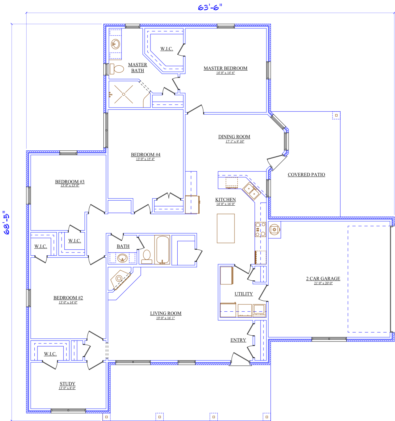
FLOOR PLAN
