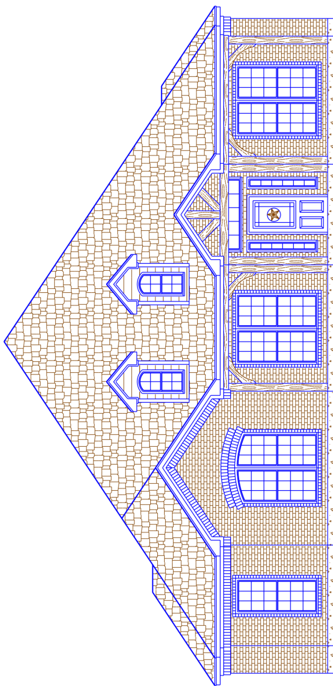
FRONT ELEVATION
