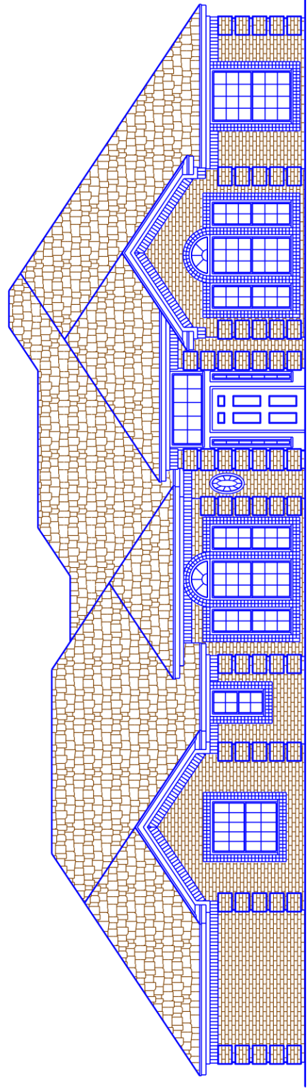
○ FRONT ELEVATION
