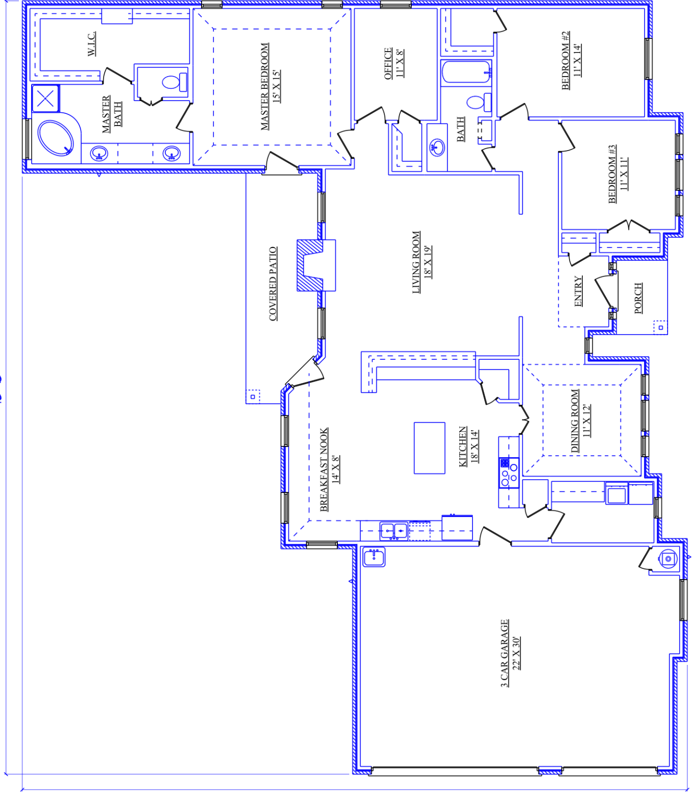
FLOOR PLAN
