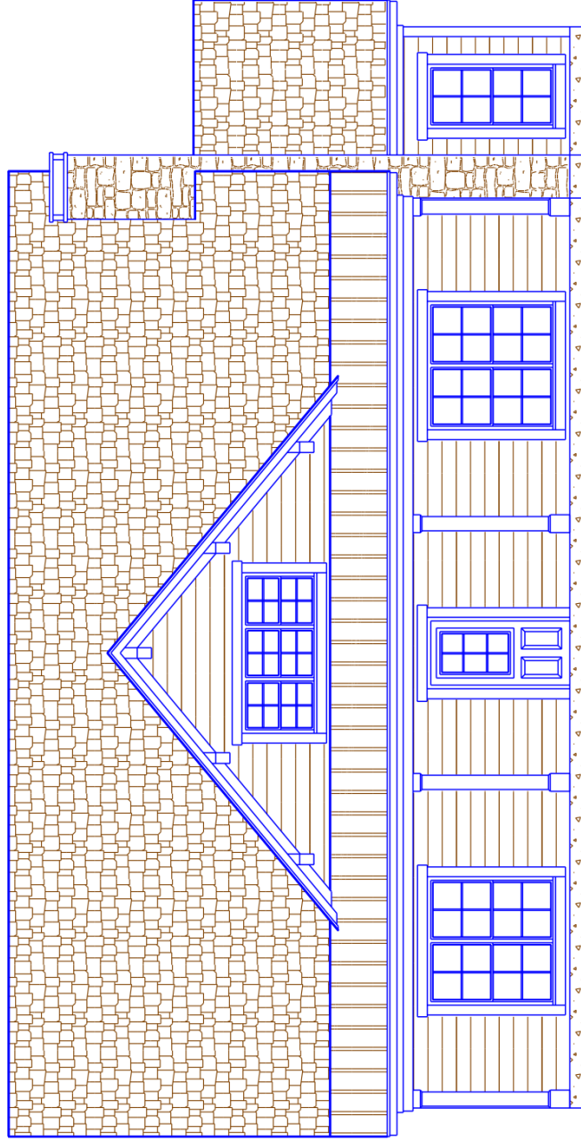
FRONT ELEVATION
