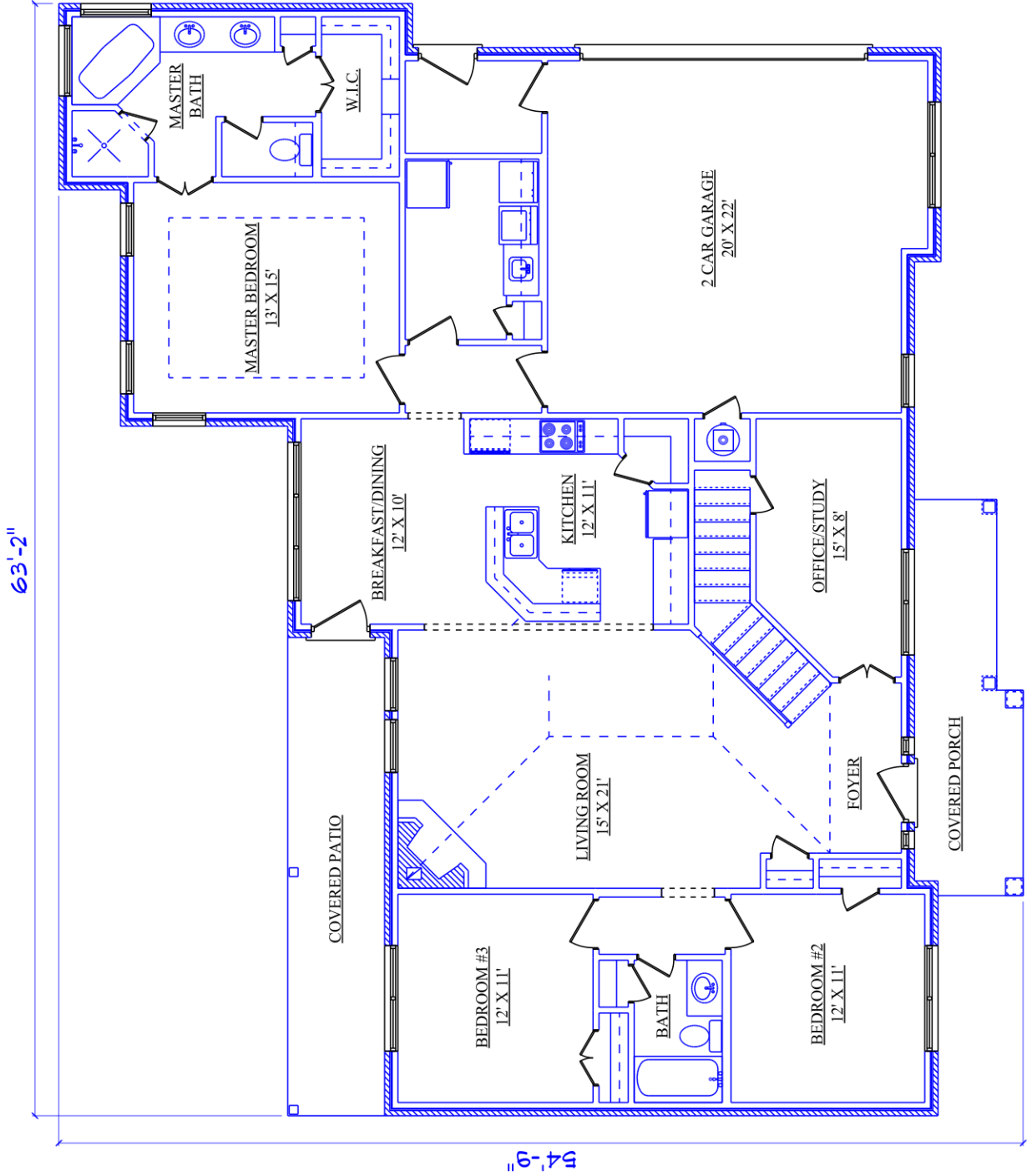
FLOOR PLAN
