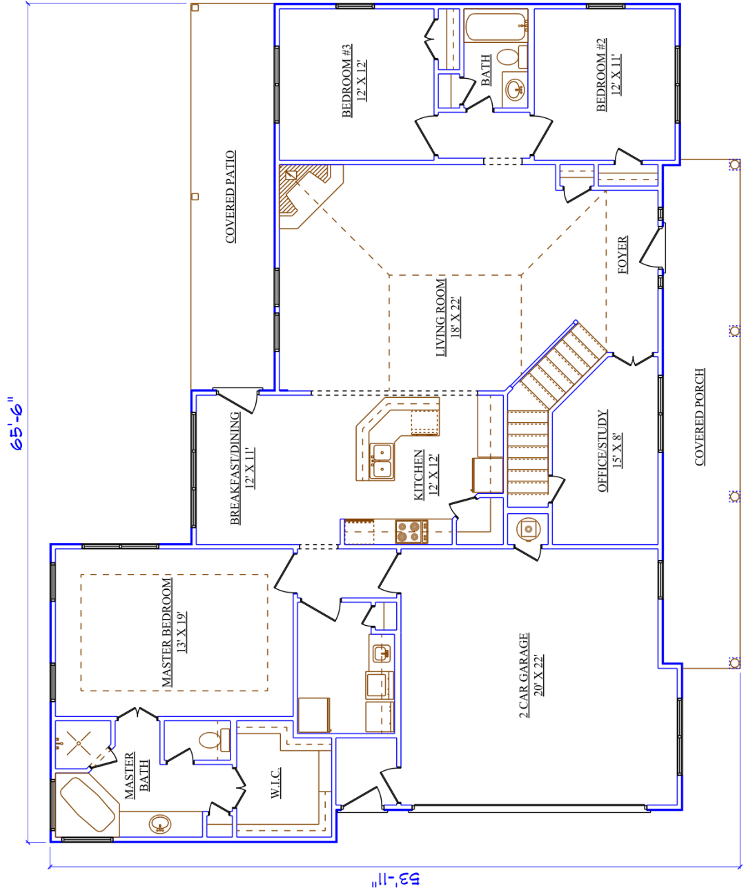
FLOOR PLAN
