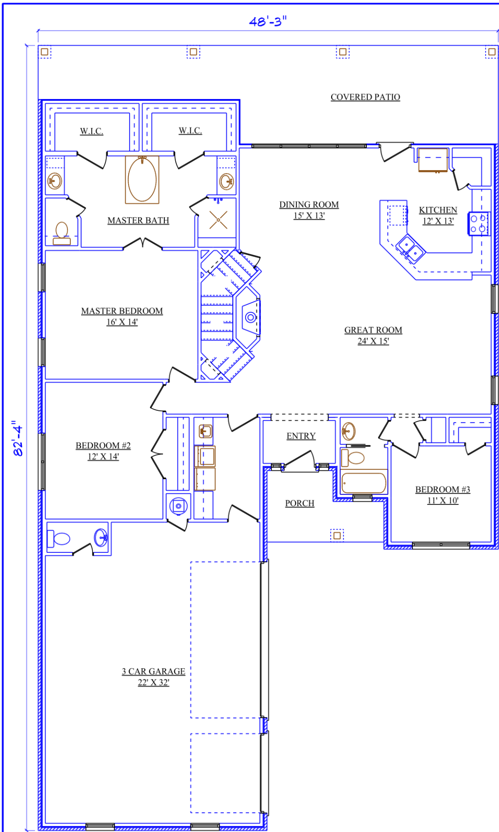
○ FLOOR PLAN
