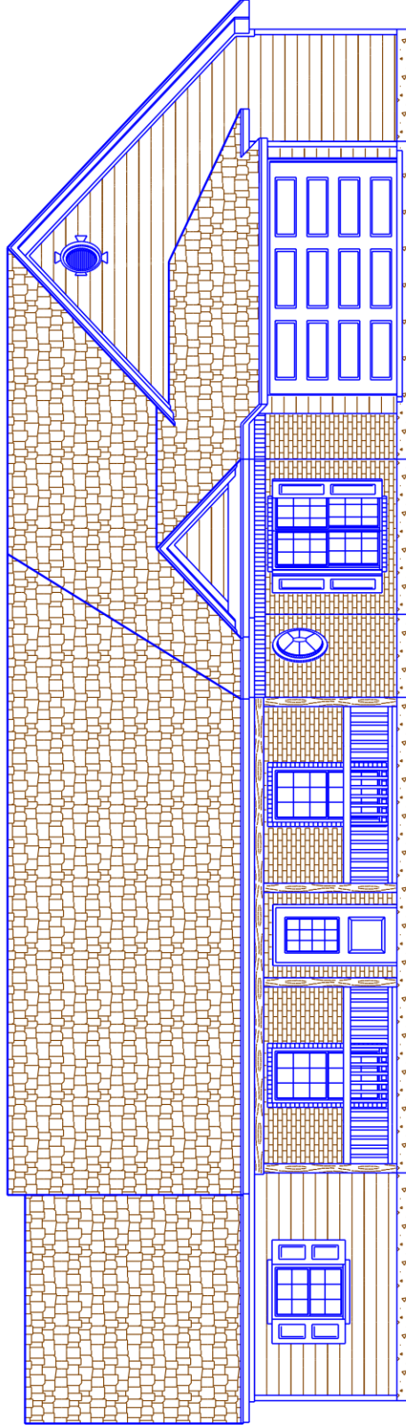
FRONT ELEVATION
