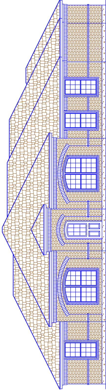
FRONT ELEVATION
