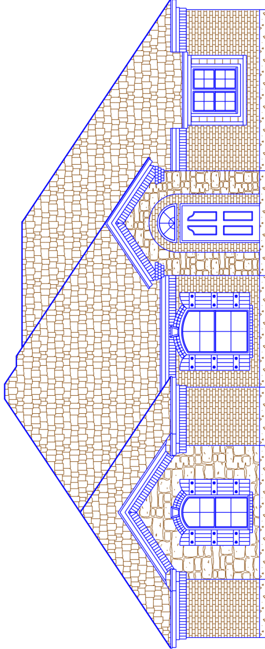
FRONT ELEVATION
