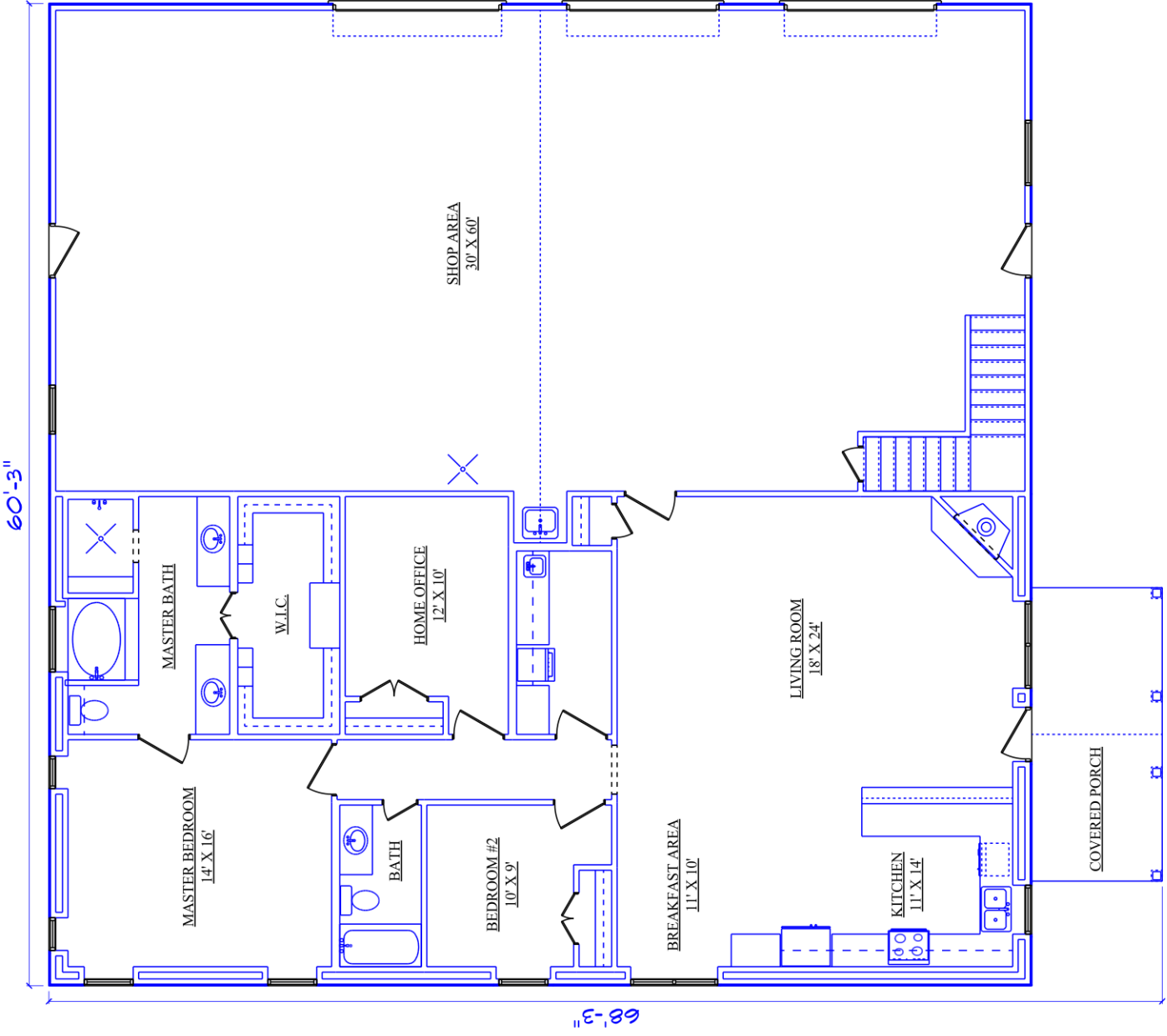
FLOOR PLAN
