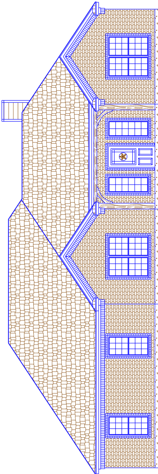
FRONT ELEVATION
