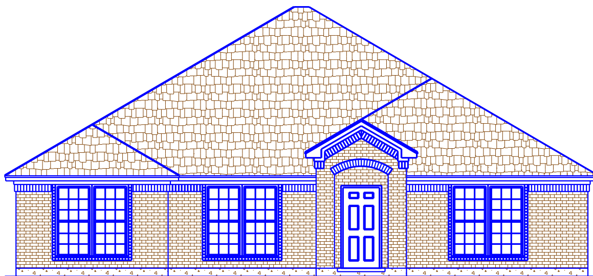
B FRONT ELEVATION
