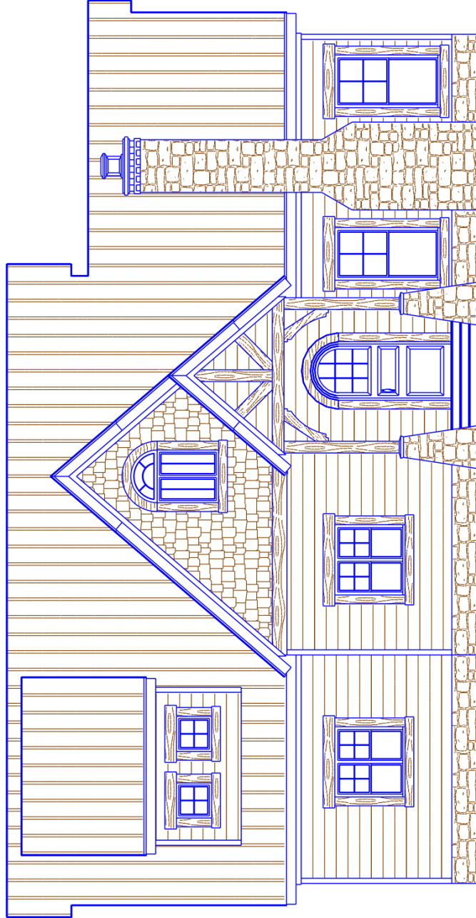
FRONT ELEVATION
