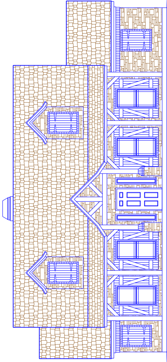
FRONT ELEVATION
