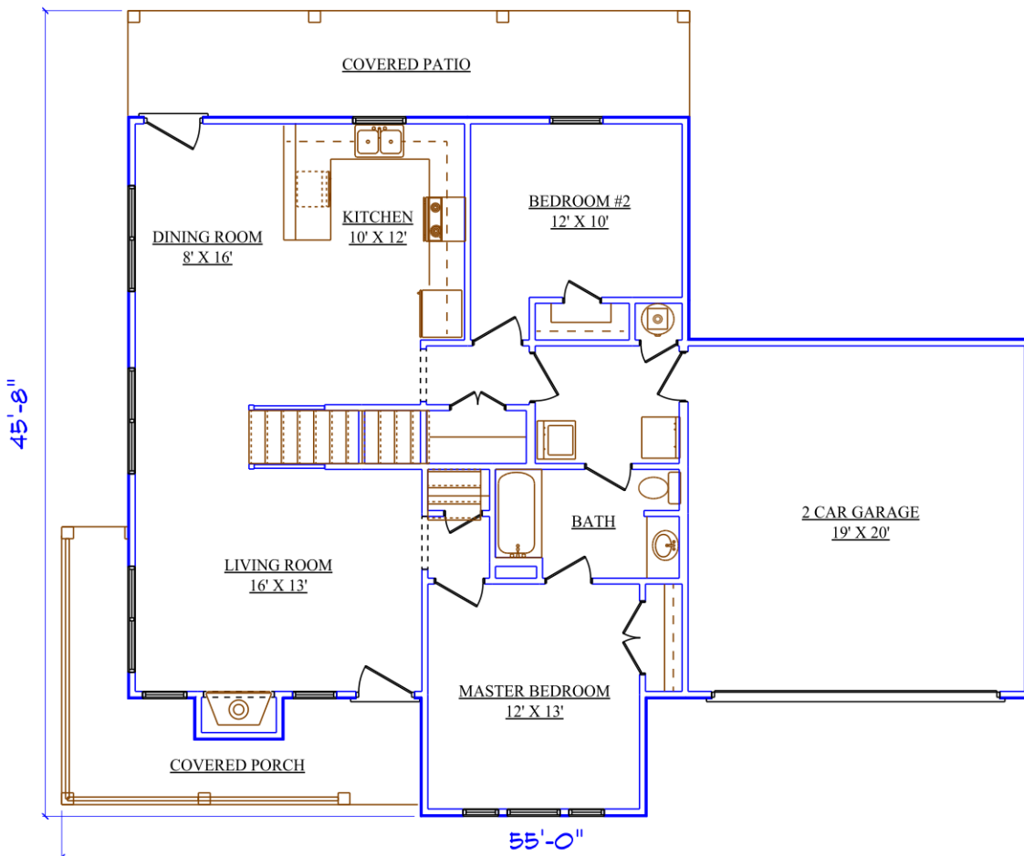
○ FLOOR PLAN
