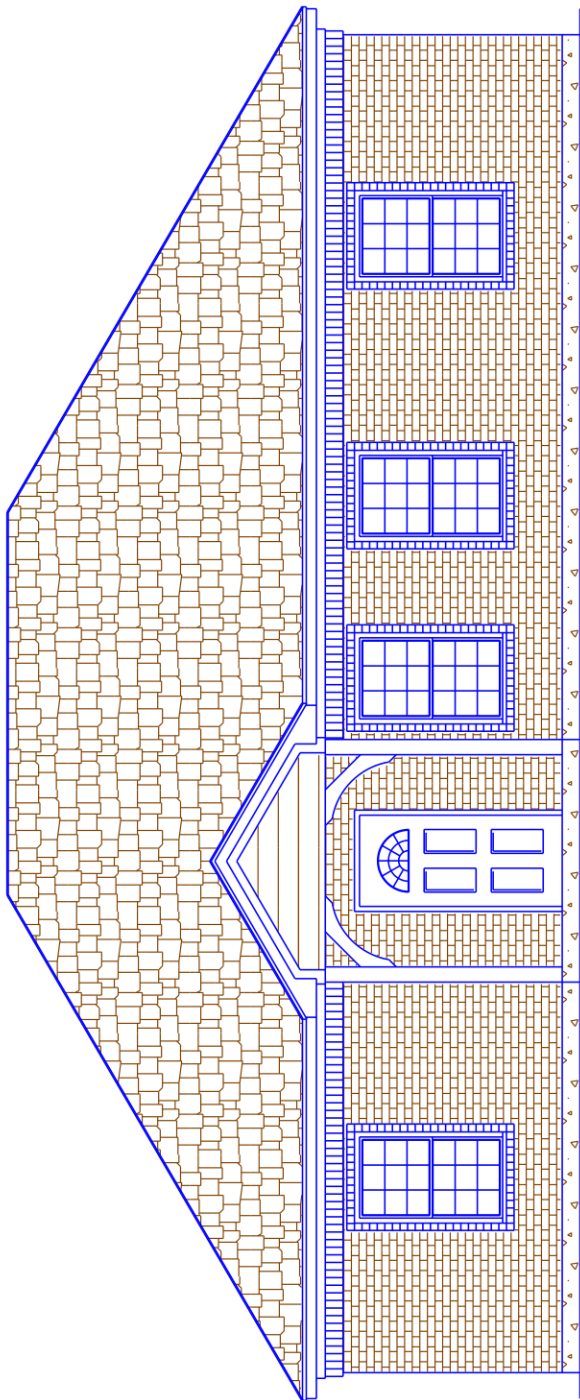
FRONT ELEVATION
