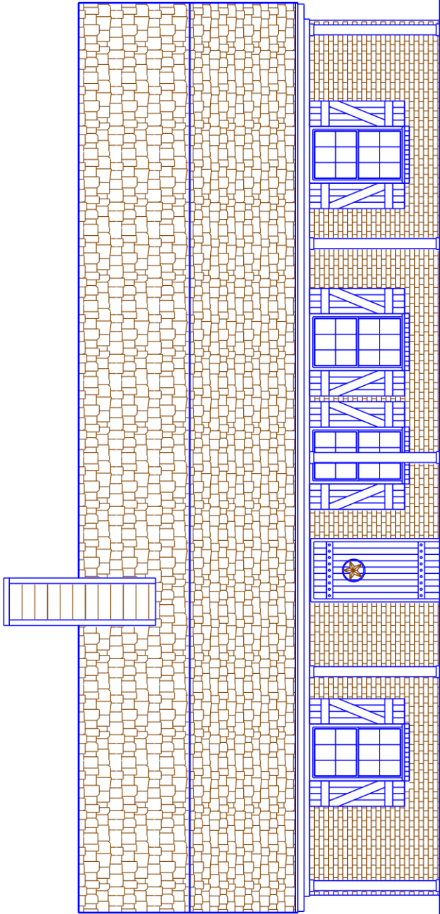
FRONT ELEVATION
